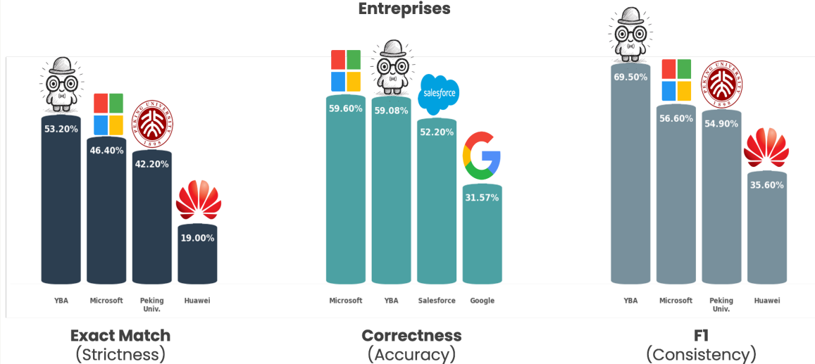
Benchmark RAGAS MuSiQue – Contextual AIs for Enterprises
